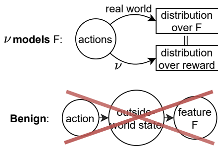
Fig. 4. Illustration of Definitions 3 and 4.
