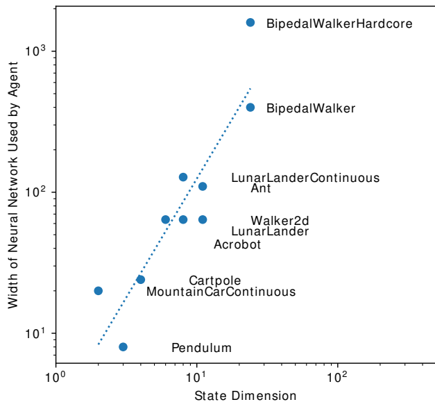
Fig. 5. Memory used to model environments of various sizes. Each data point represents the most space-efficient, better-than-average, neural-architecture-using agent on the OpenAI Gym Leaderboard for various environments.
