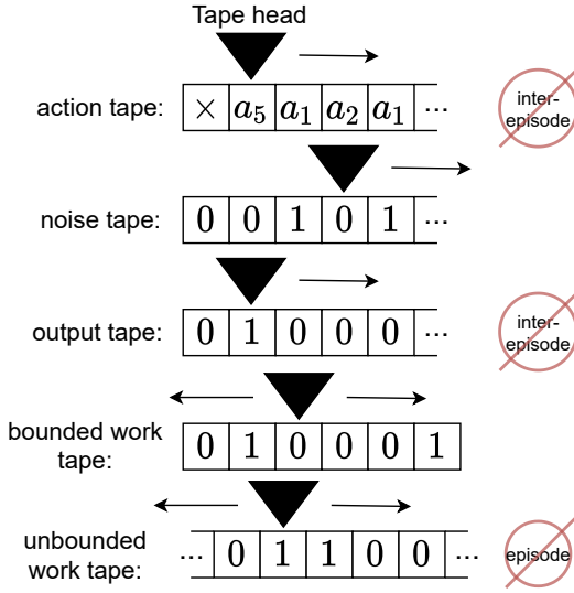
Fig. 3. A space-bounded Turing machine architecture. During the episode phase, the unbounded work tape head cannot move. During the inter-episode phase, the output tape head cannot move or write, and as soon as the action tape head moves, the inter-episode phase is over. This architecture is designed to restrict space-intensive computation during the episode phase.
