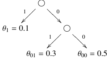
Figure 1: An example prediction suffix tree
