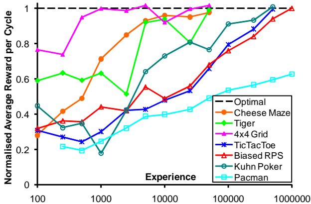
Figure 2: Learning scalability results
